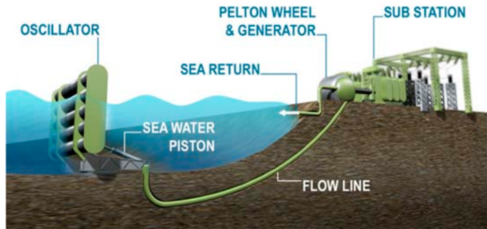
Aquamarine Power Oyster ( http://www.aquamarinepower.com )
