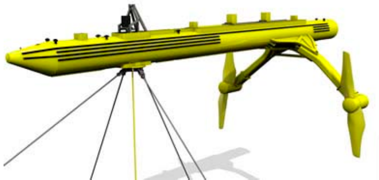
Scotrenewable ( http://www.scotrenewables.com/ )
