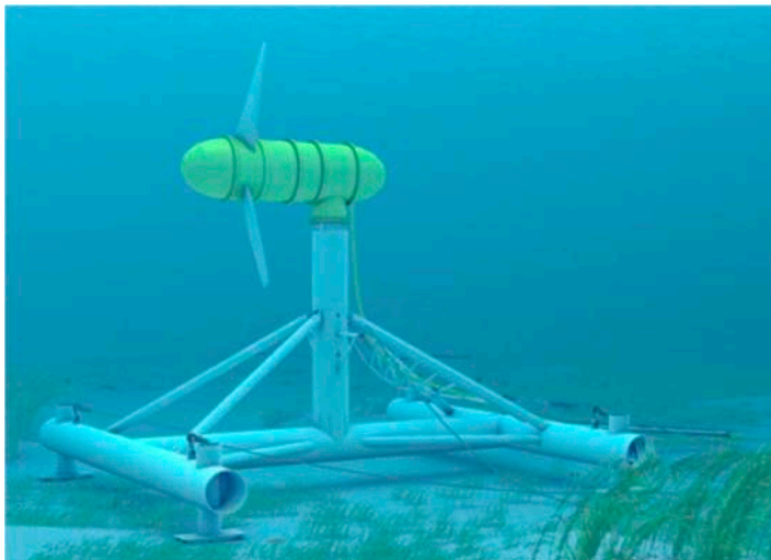
Voith Hydro HyTide ( http://www.voith.com/en/products-services/hydro-power/ocean-energies/tidal-current-power-stations--591.html )
